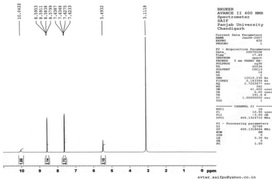
Figure 2. ^1\text{H} NMR spectra.
