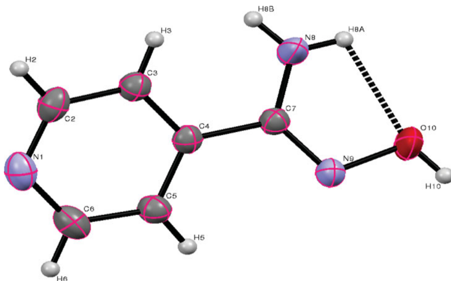
Figure 5. ORTEP view of the title molecule with atom numbering scheme. The displacement ellipsoids for nonhydrogen atoms are drawn at 50% probability level. Dashed line indicates intramolecular hydrogen bond of the type N—H...O.
