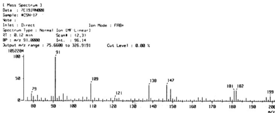
Figure 3. FAB mass spectrum.
