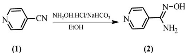
Scheme 1. Synthesis of Compound (Z)-2- N' -hydroxyisonicotinamidine.
