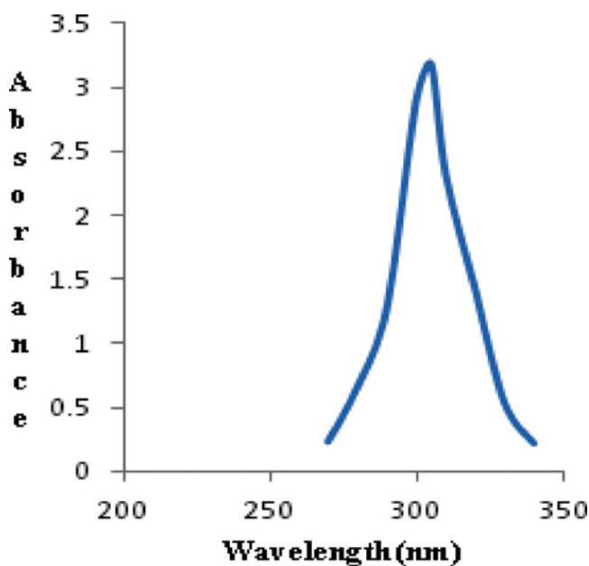
Figure 4. UV-visible spectrum.
