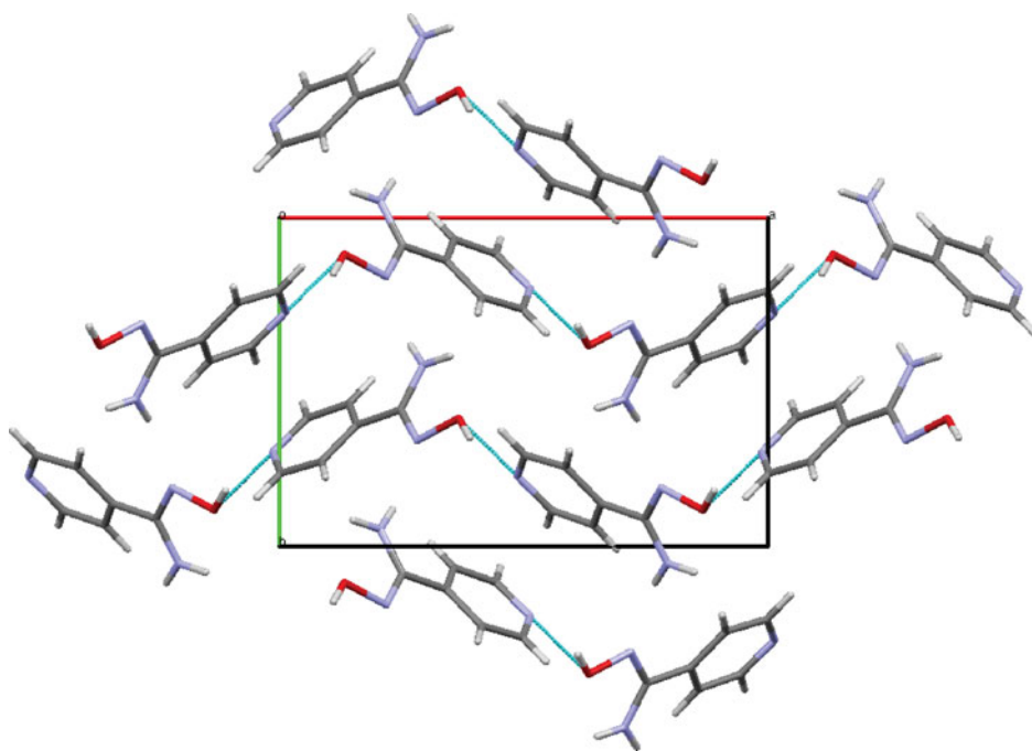
Figure 8. Packing of molecules when viewed down the c -axis.
