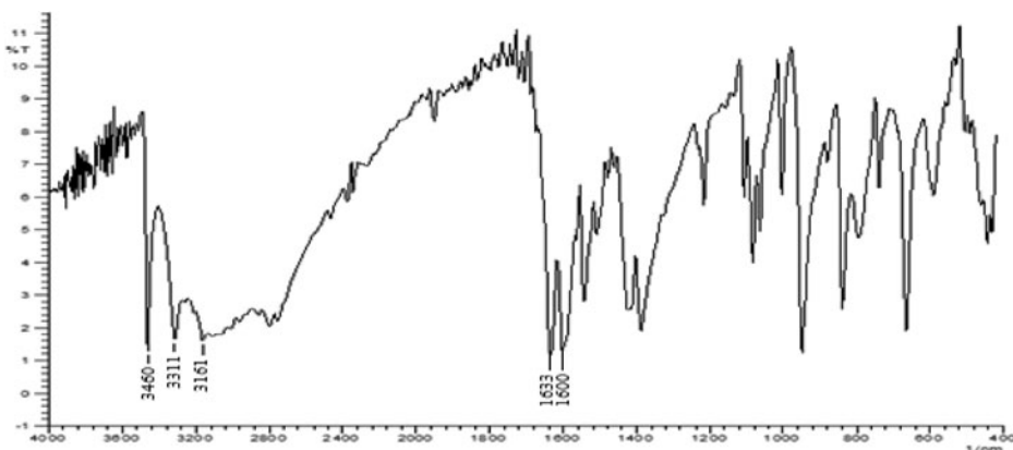
Figure 1. FT-IR spectrum.
